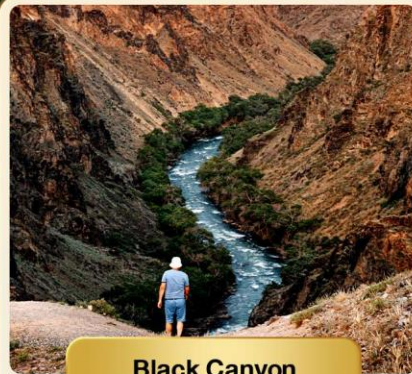
Black Canyon
