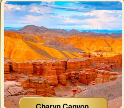
Charyn Canyon
